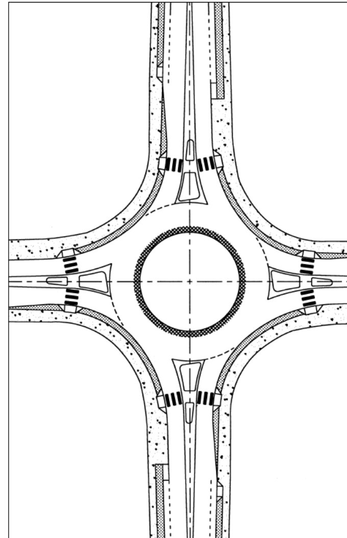
Single-Lane Roundabout
