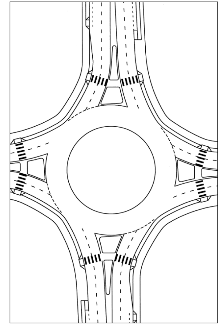
Double-Lane Roundabout
